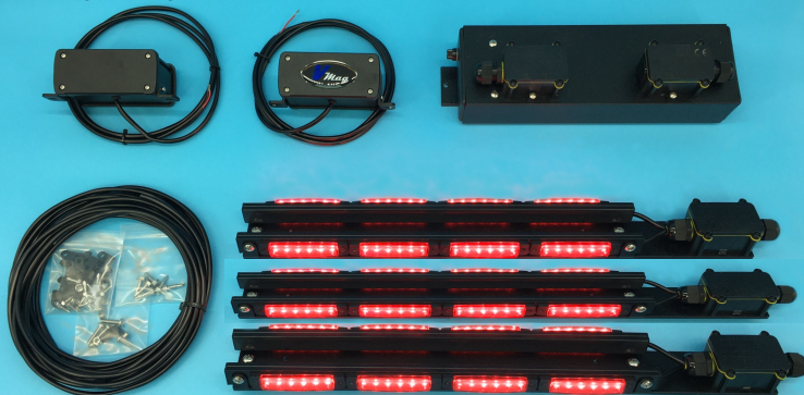
POWER RECEIVER
